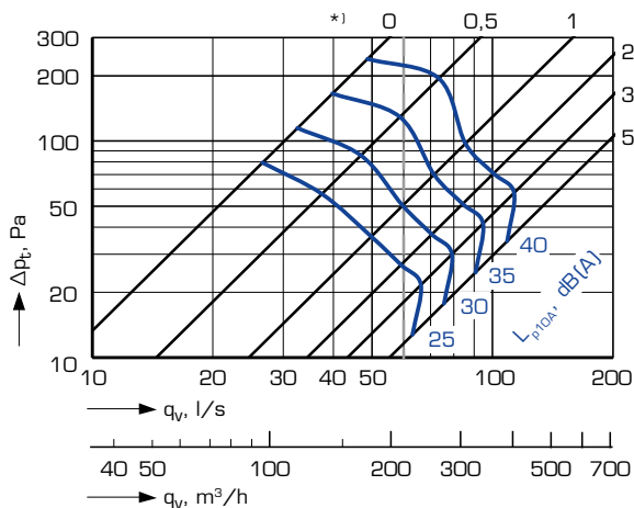
DYVB-200-1 WITH CONNECTION FROM THE REAR
